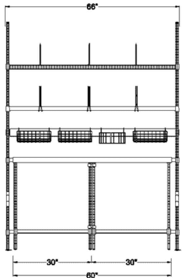
FRONT ELEVATION
