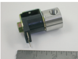
Roundup Solenoid Valve #ROU4040145
