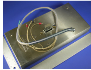
Dough Pro Upper Platen Assy - Right #DPR11090131R100
