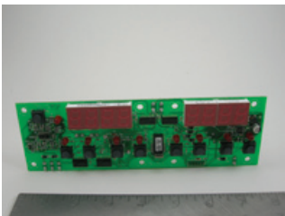
Star Mfg. Time/Temp Control Board #STAZ3263
