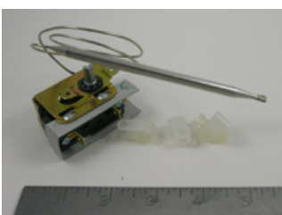
Henny Penny Thermostat w/Clips 160-210 Degree #HEN14209
