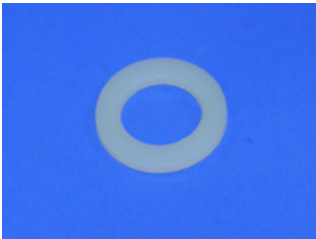
Middleby Marshall Nylon Spacer 1-1/4 OD 3/4 ID #MID35000-1080
