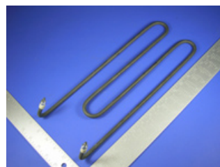
Bevles Element 120V 1800W #BVL784676
