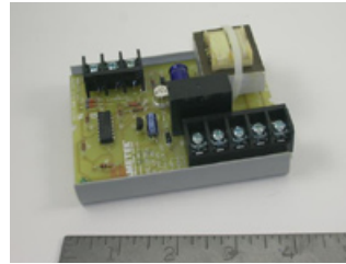
Delfield Solid State Control Relay #DEL2193994
