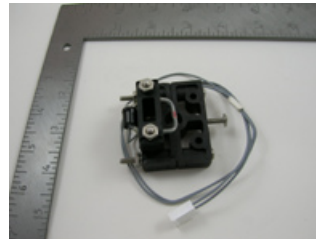
Bunn-O-Matic Thermister Assy 240V #BUN12586.0000
