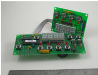
Dough Pro Digital Controller #DPR110888052
