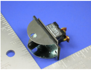
Dough Pro Power Switch Kit #DPR110901410
