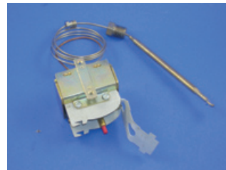
Pitco Hi Limit Thermostat Gas #PITPP10084
