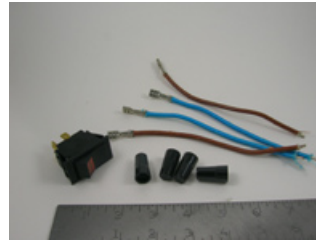
Cres Cor On/Off Switch Kit 120V 20A #CRE0808-113-K
